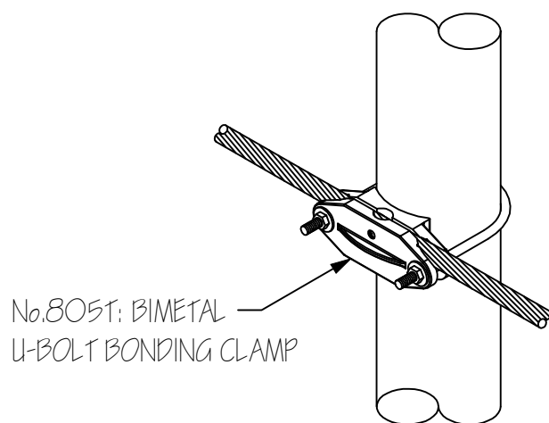
No. 805T: BIMETAL U-BOLT BONDING CLAMP
