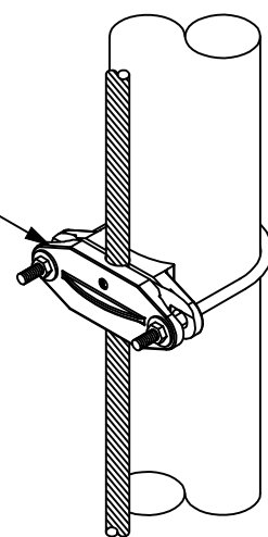
No. 805T: BIMETAL U-BOLT BONDING CLAMP
