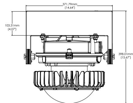
YOKE MOUNT 0-90° (YK90)
