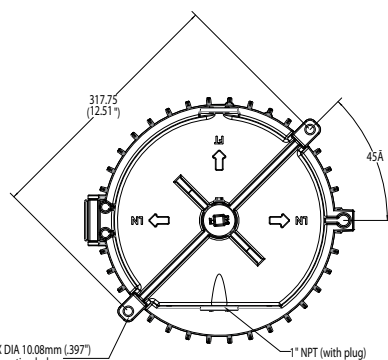
CEILING MOUNT (UNM)
