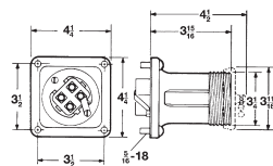
AR receptacle - open and with cap
