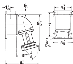
ARE assembly
